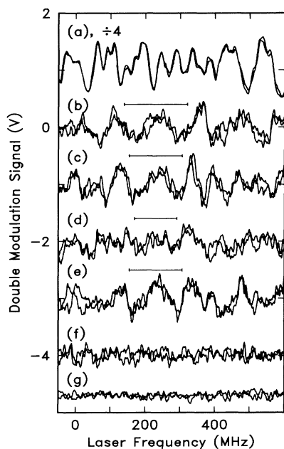
FIG. 2. Examples of single-molecule spectra using the FMUS technique. (a) Traces of SFS at the O_1 line center, 592.312 nm, 128 averages each. (b) SMD spectra at 592.469 nm, \nu_m = 91 \text{ MHz} , 128 averages, bar shows the value of 2\nu_m . (c) \nu_m = 76 \text{ MHz} . (d) \nu_m = 61 \text{ MHz} . (e) Back to \nu_m = 76 \text{ MHz} . (f) Far off line at 590.462 nm. (g) No light on the detector.
