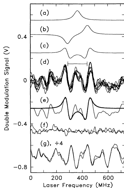
FIG. 1. Illustration of single-molecule spectra using FMS technique. (a) Simulation of absorption line, \gamma = 65 MHz. (b) Simulation of FM spectrum for (a), \nu_m = 75 MHz. (c) Simulation of FMS line shape. (d) SMD spectra at 592.423 nm, 512 averages, 8 traces overlaid, bar shows value of 2\nu_m = 150 MHz. (e) Average of traces in (d) ( S_2 removed) with fit to the in-focus molecule (smooth curve). (f) Signal far off line at 597.514 nm. (g) Traces of SFS at the O_2 line center, 592.186 nm.
